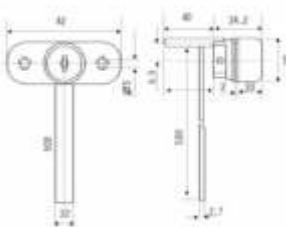
central Locking 122cm, 61cm
